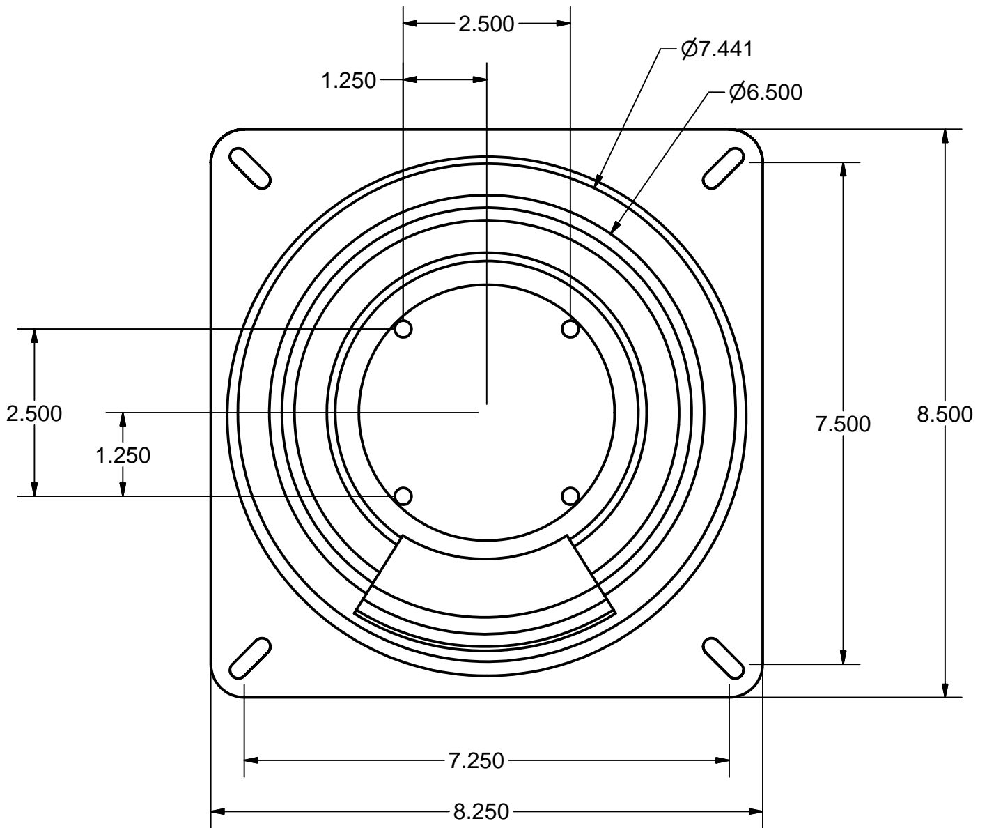
BOTTOM VIEW
